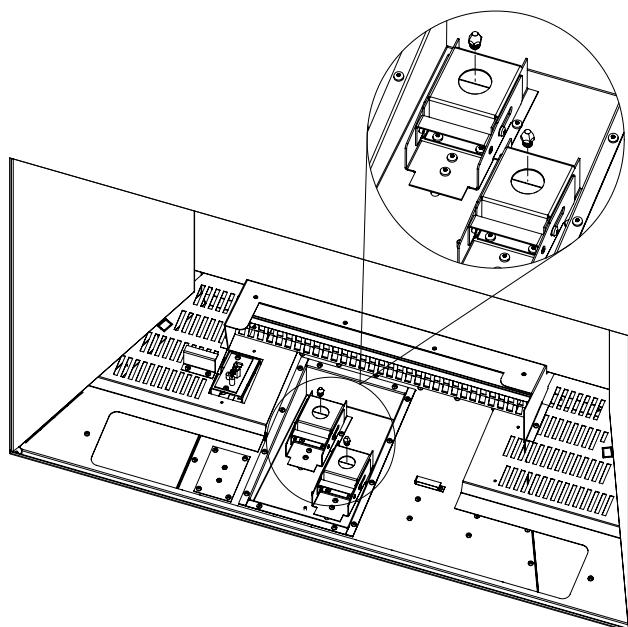
Figure 27: Emplacements D'orifice
