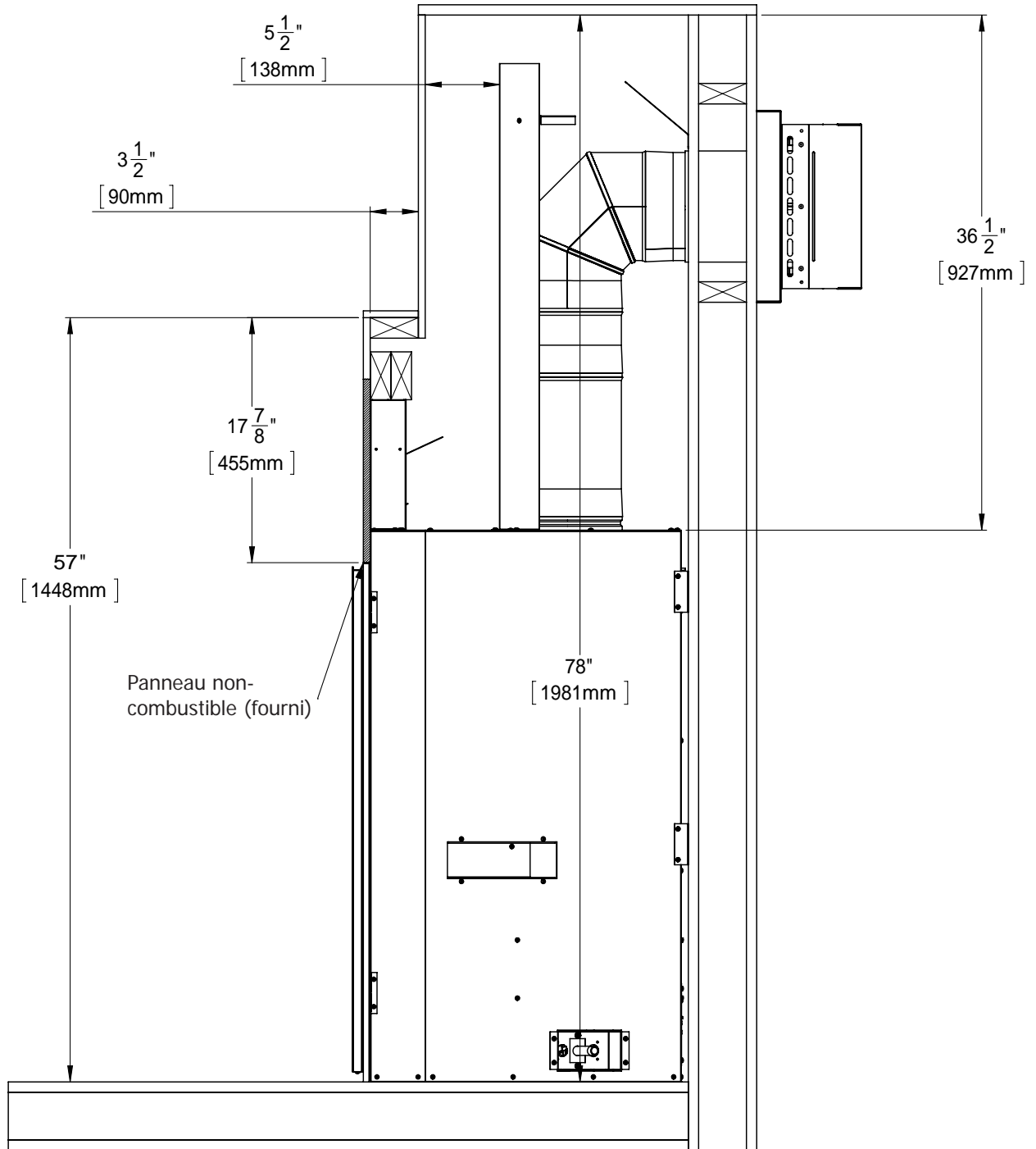
Figure 51: Installation Encastrée
