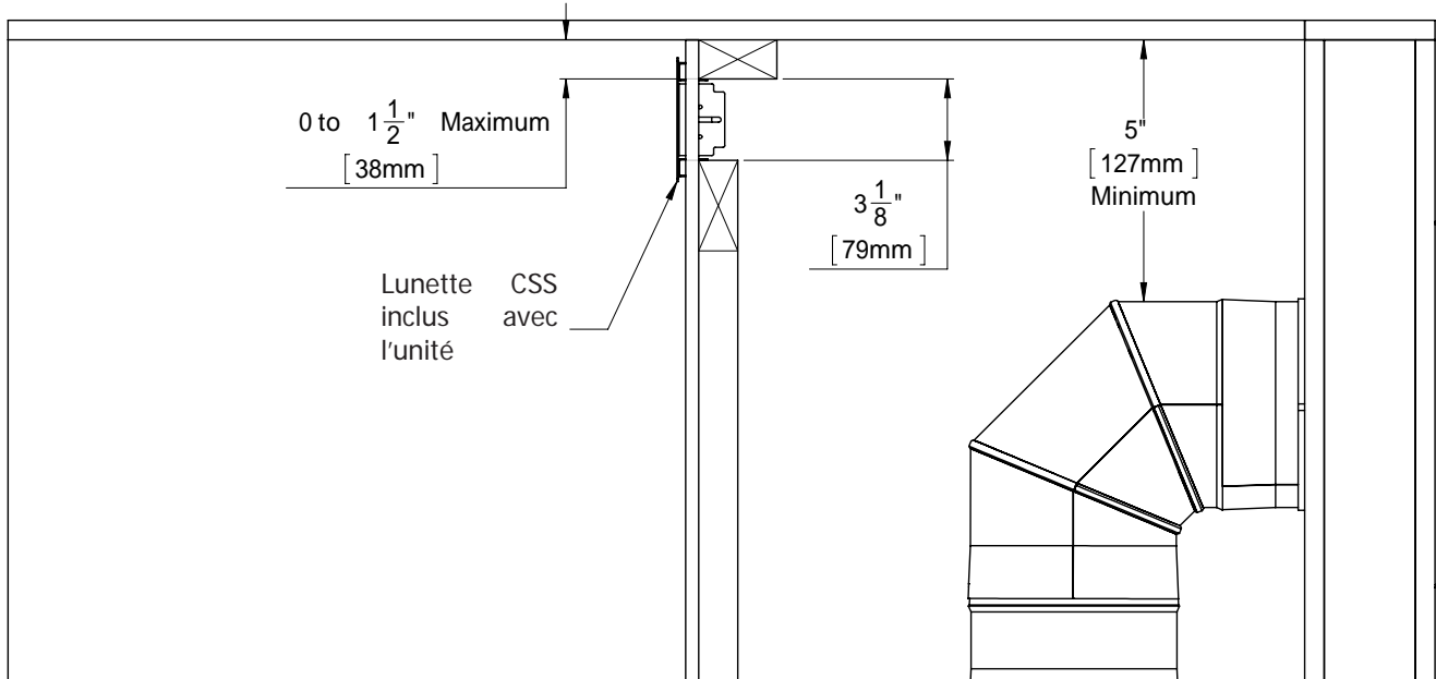
Figure 46: Encadrement Option 3
