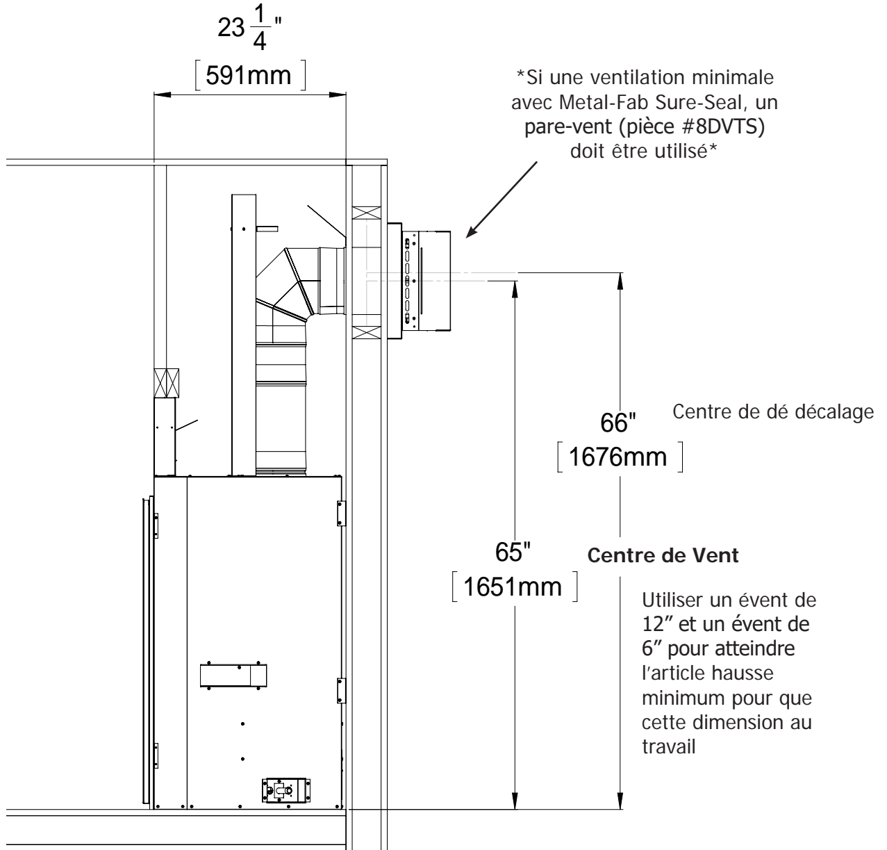
Figure 53: Fente Minimum
