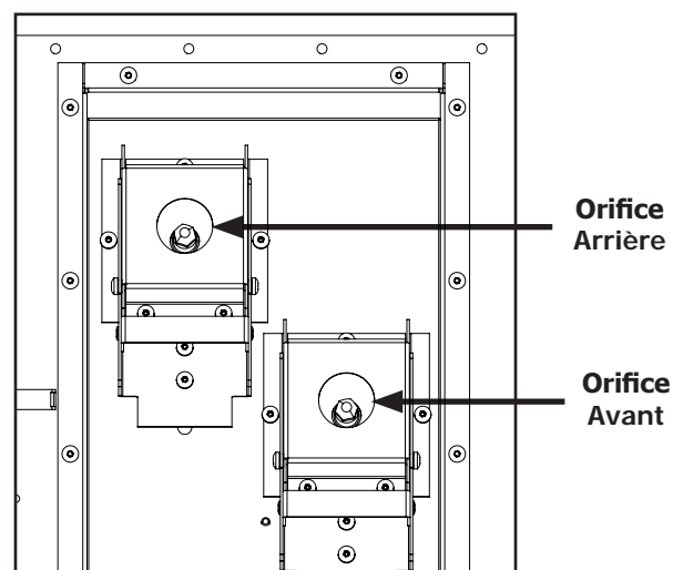
Figure 28: Emplacements D'orifice
