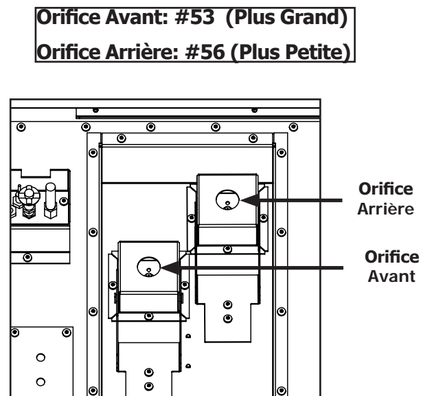
Figure 28: Emplacements D'orifice
