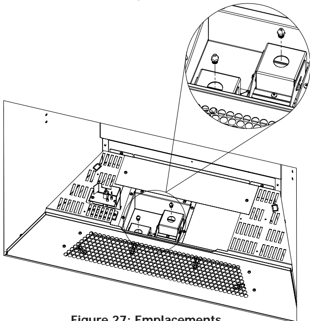
Figure 27: Emplacements D'orifice
