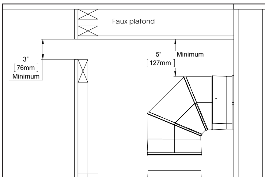
Figure 53: Faux Plafond
