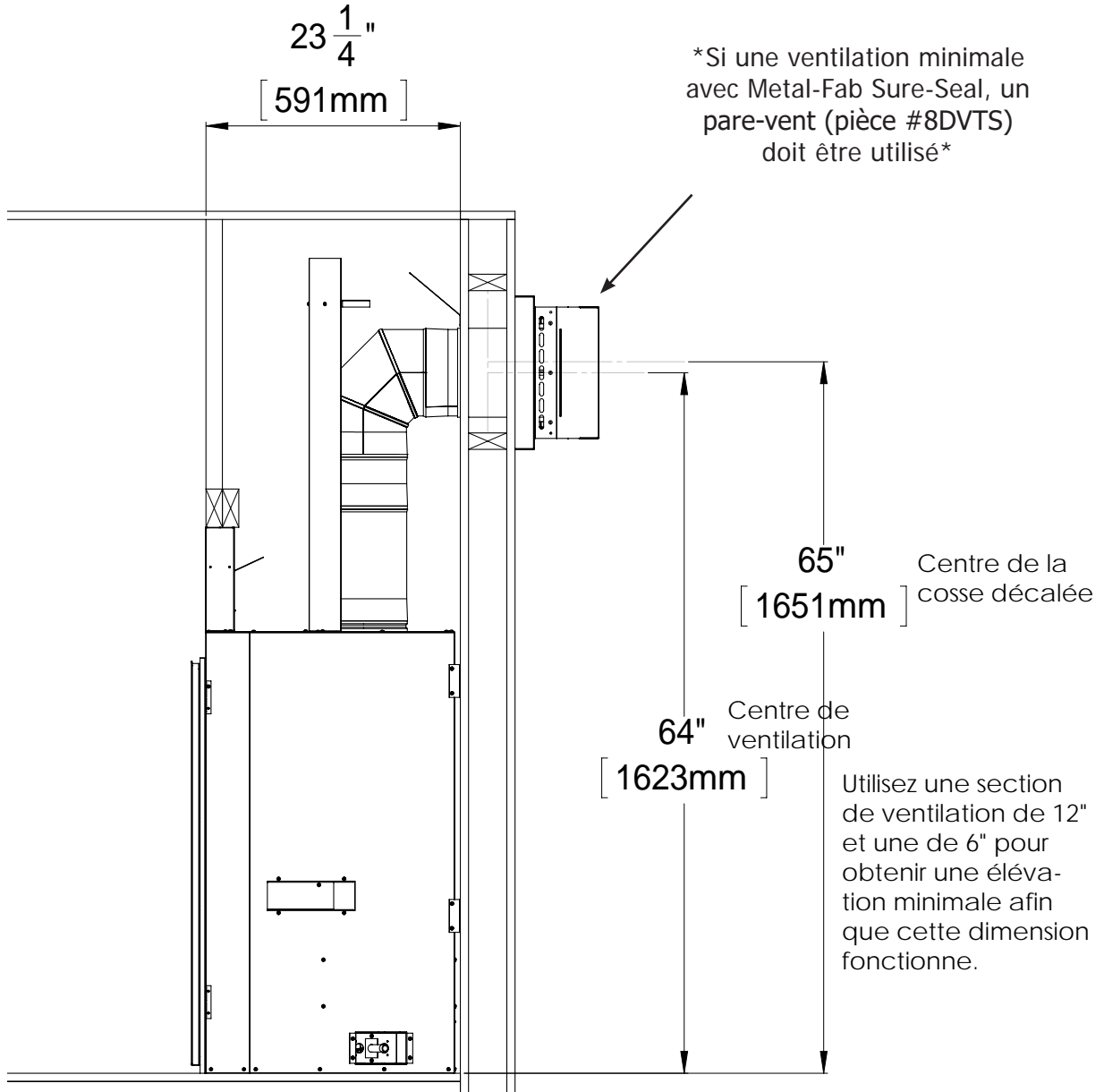
Figure 59: Fente Minimum
