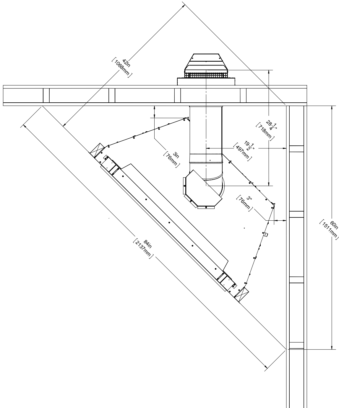
Figure 57. Installation en Coin
