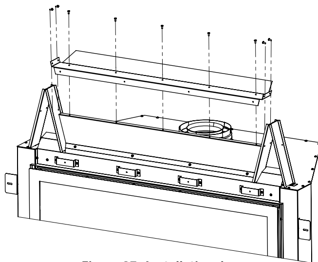
Figure 37: Installation de Contreventement
