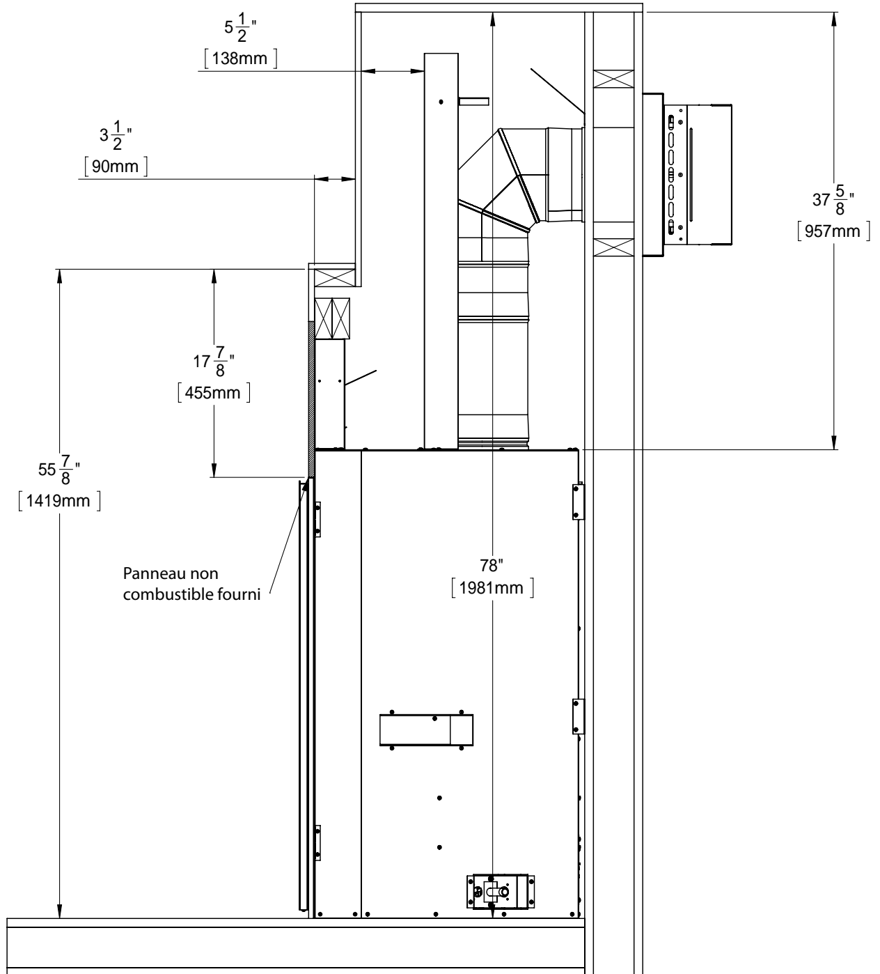
Figure 56: Installation Encastrée
