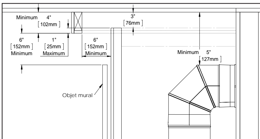
Figure 49: Installation de Cantonnière
