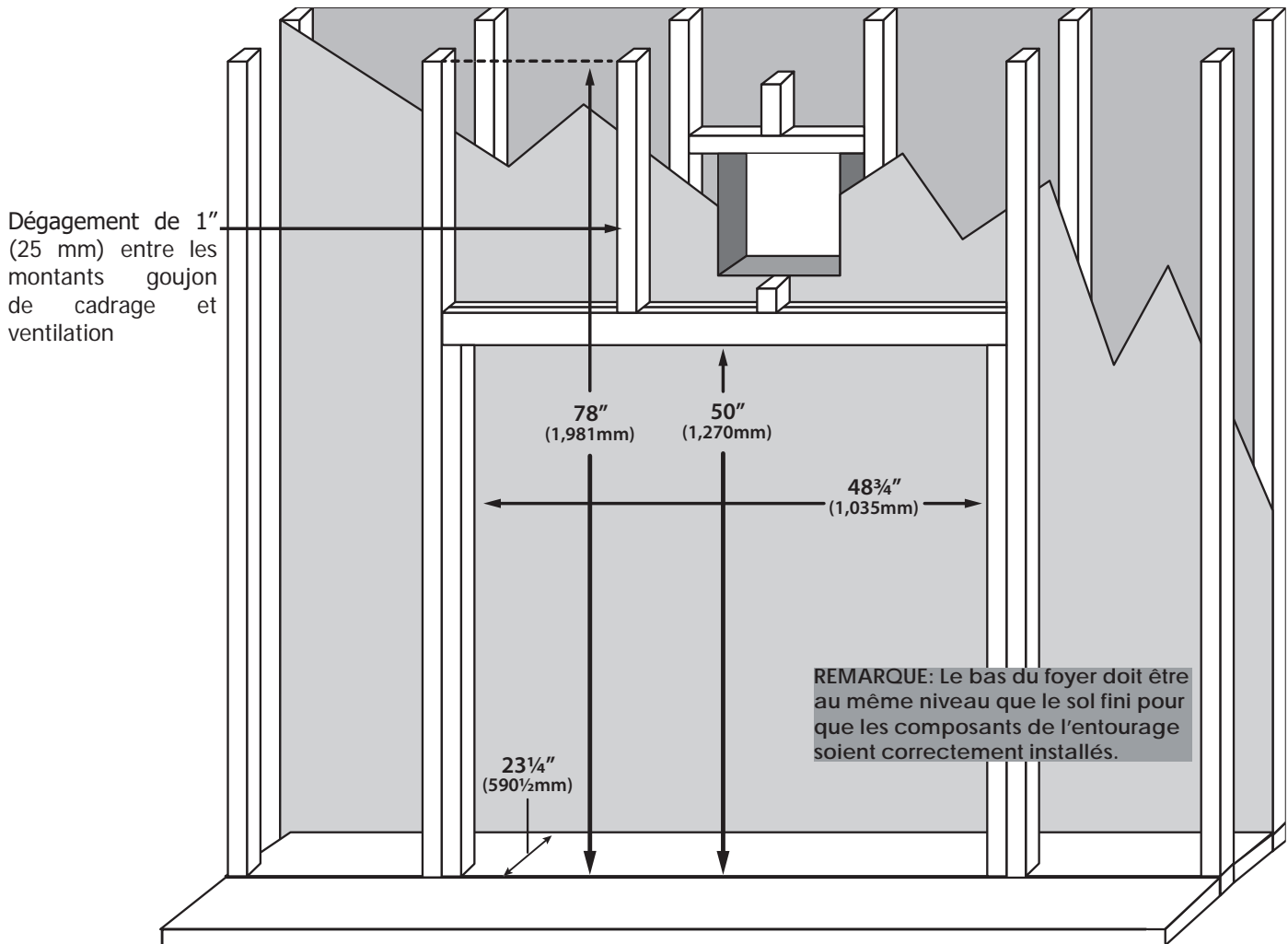
Figure 40: G42 Encadrement Minimum
