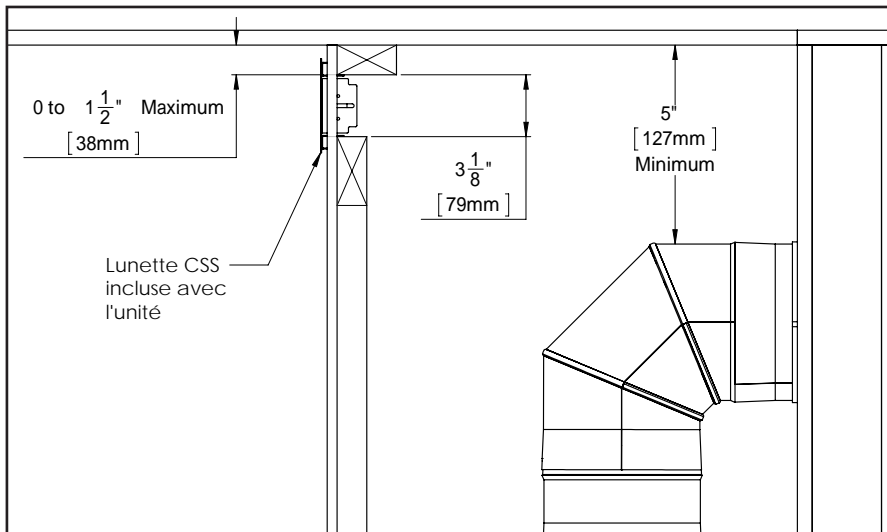
Figure 51: Option de Cadrage 3
