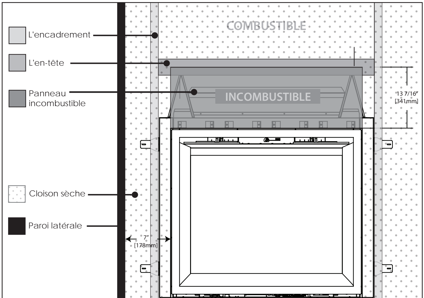
Figure 61. Typical Facing Layout
