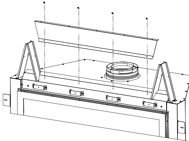
Figure 36: Installation de Support de Bouclier Thermique
