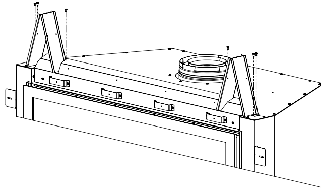
Figure 35: Installation de Impasse Haute
