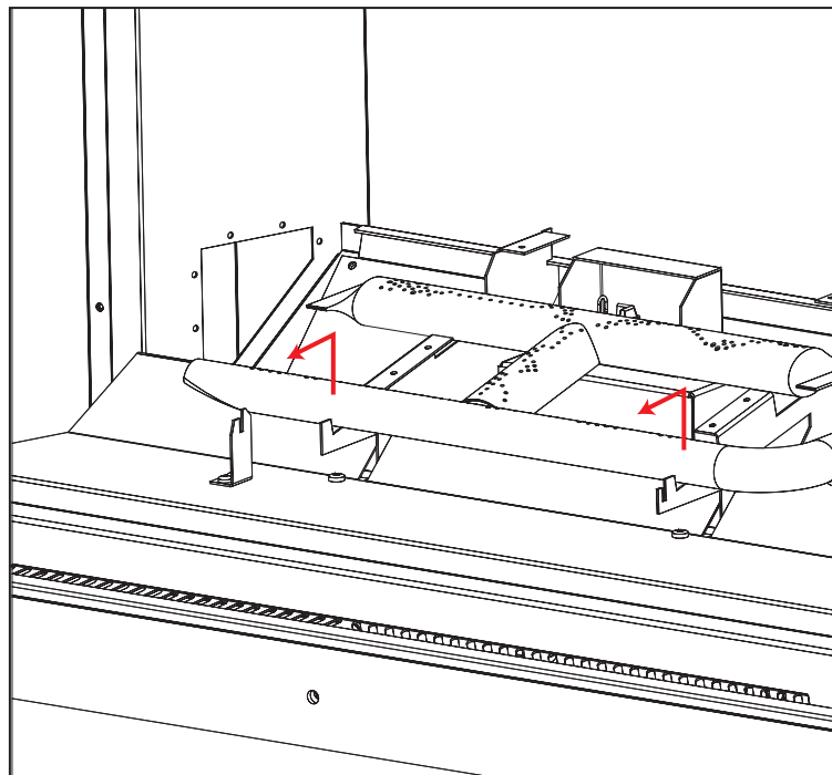
Figure 10. Retrait Burner
