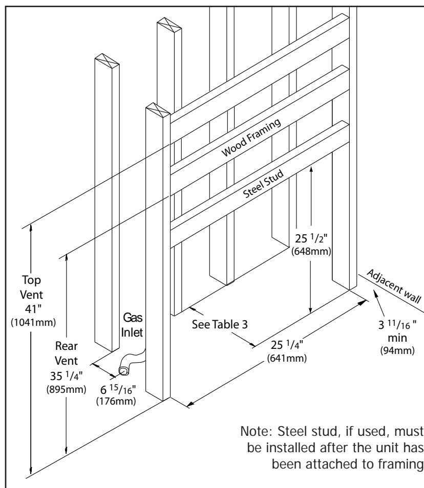
Figure 23: Minimum Framing Dimensions
