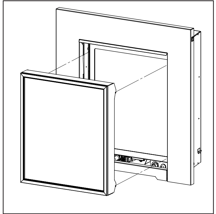
Figure 70: Installing Safety Screen onto Cabinet Bracket
