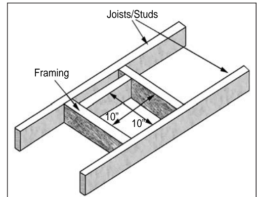
Figure 38: Vent Thimble Framing
