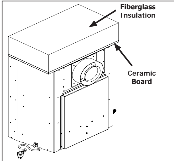
Figure 26: Unit Insulation - Rear Vent
