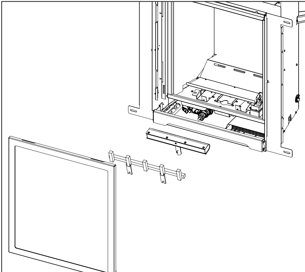
Figure 19: Burner Removal
