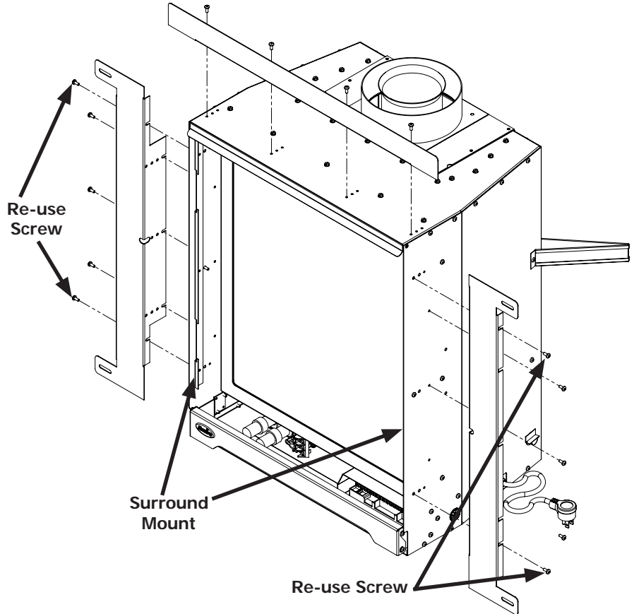
Figure 32: Tiling Flange Installation
