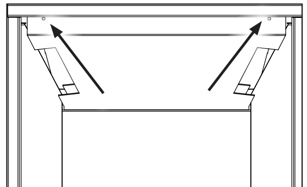
Figure 68: Top Liner Screws (Porcelain Liners only).
