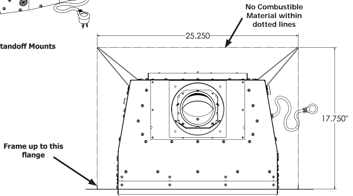
Figure 29: Area created by standoffs
