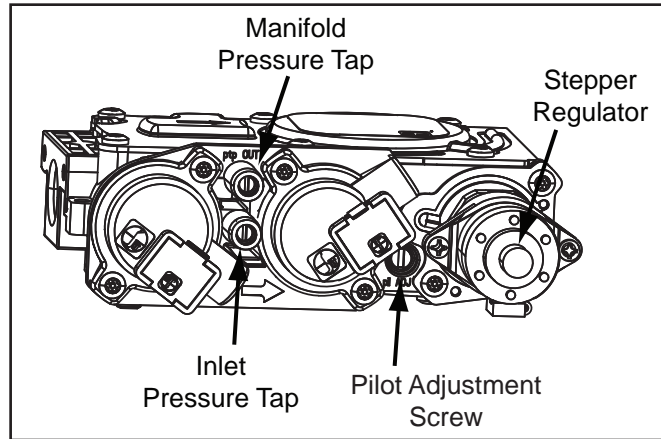
Figure 56: Fully Labeled Gas Valve
