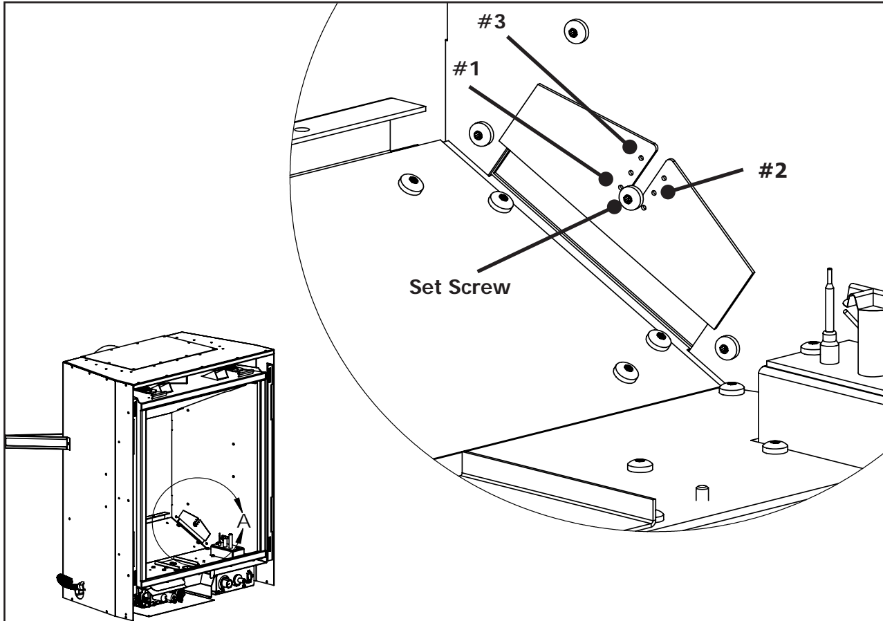
Figure 54: Installation of Air Restrictors
