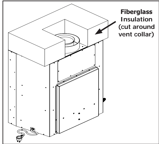
Figure 27: Unit Insulation - Top Vent
