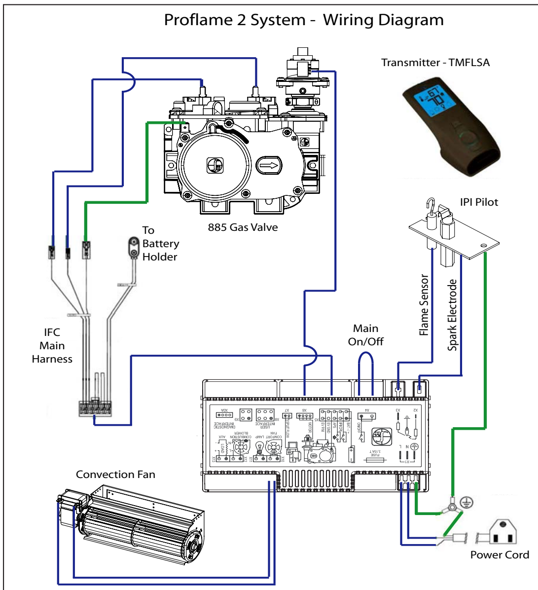
Figure 57: Wiring Diagram
