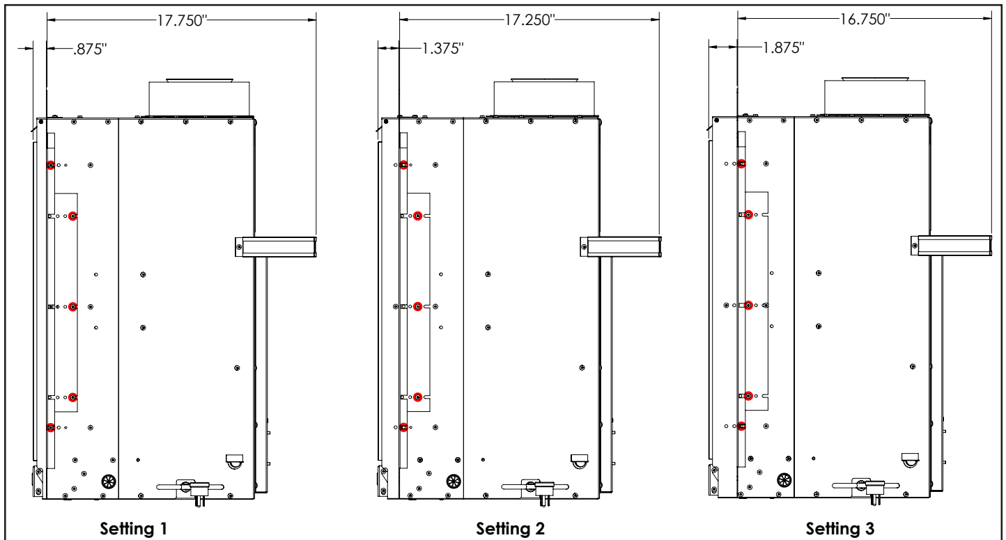
Figure 33: Tiling Flange Positions
