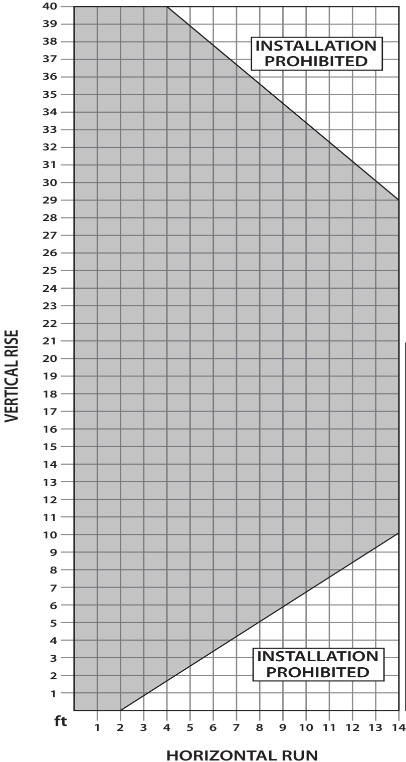
Figure 41: Possible Vent Configurations for Top Vented Vertical and Horizontal Terminations.
