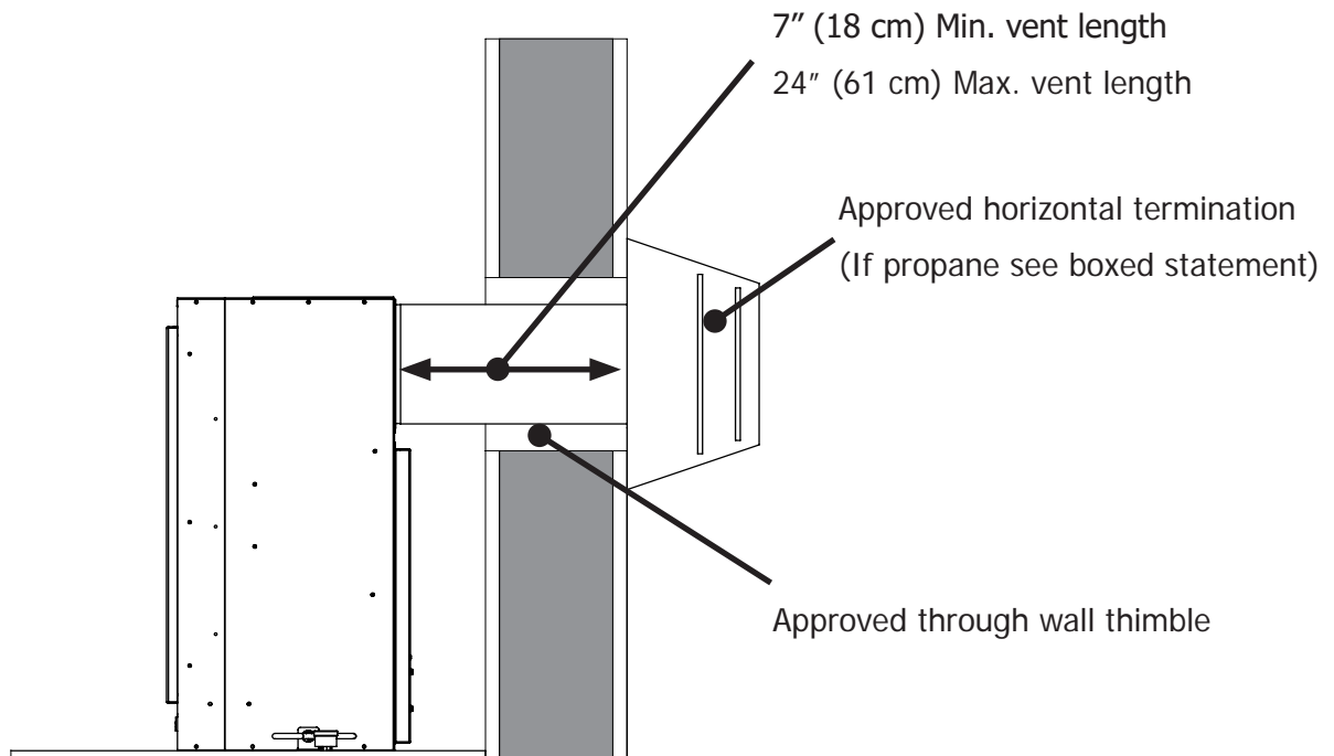
Figure 40: Flat Wall Rear Vent - No Vertical Rise
