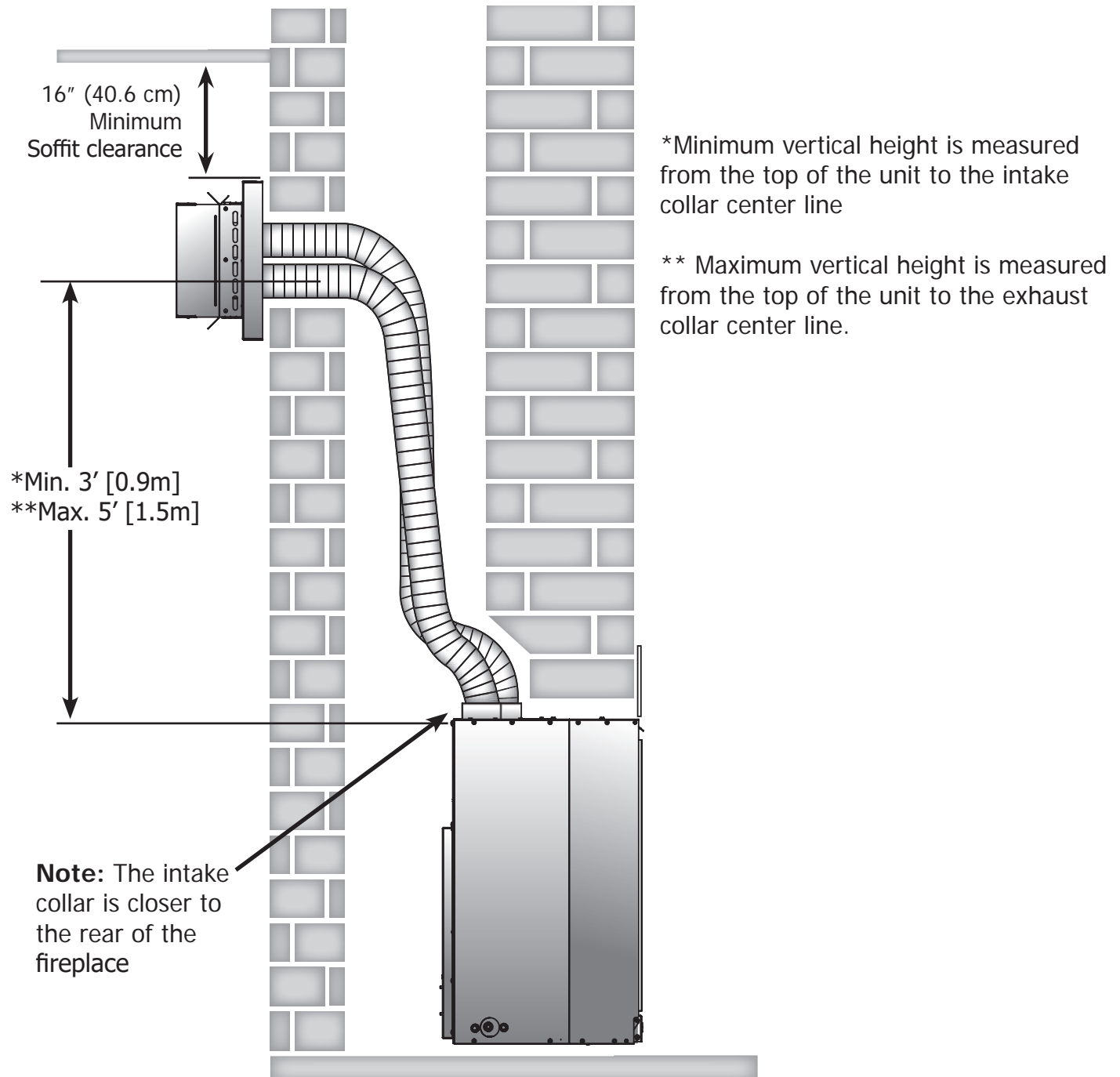
Figure 52: Min and Max Horizontal Termination
