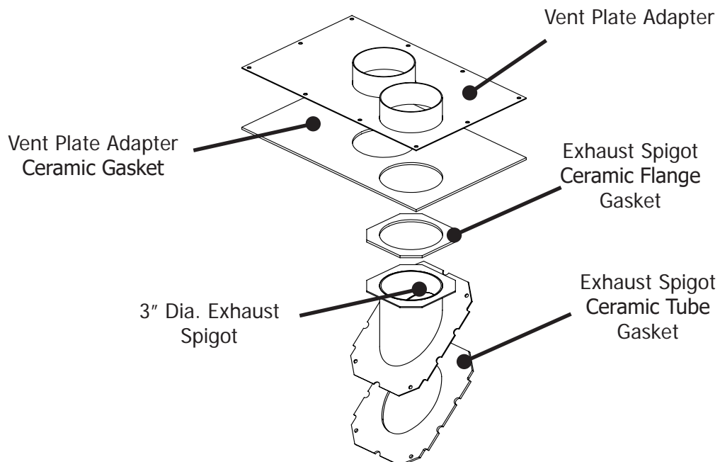
Figure 49: Q1 Co-Linear Venting Kit Contents
