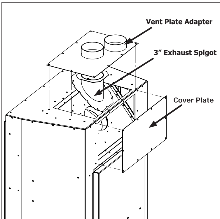
Figure 51: Installation of Co-Axial Venting parts
