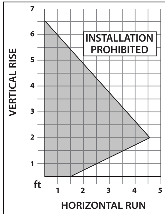
Figure 42: Possible Vent Configurations for Rear Vented Vertical and Horizontal Terminations.
