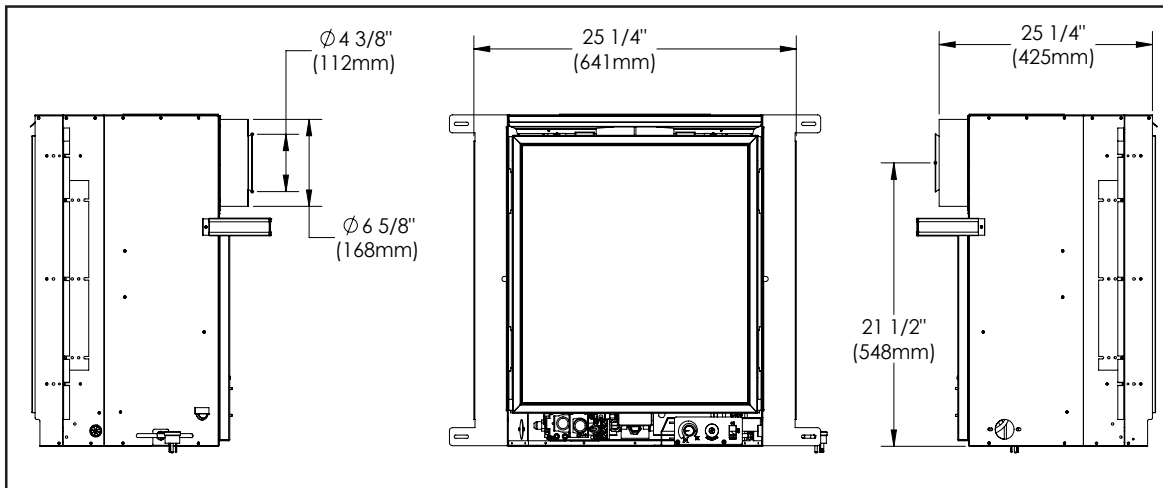
Figure 2: Q1 Dimensions - Rear Vent Configuration
