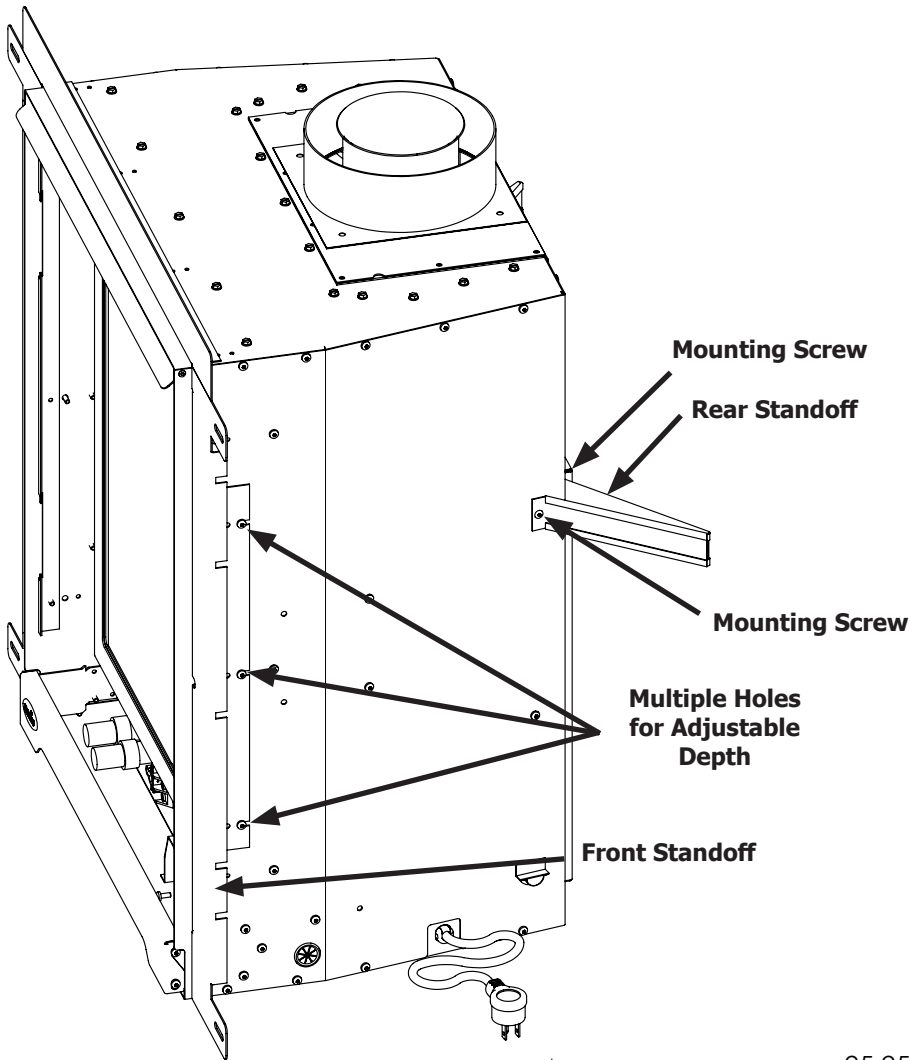
Figure 28: Standoff Mounts
