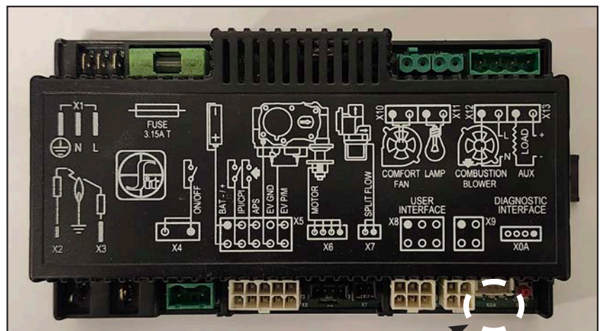
LED Location Figure 71: IFC LED Location
