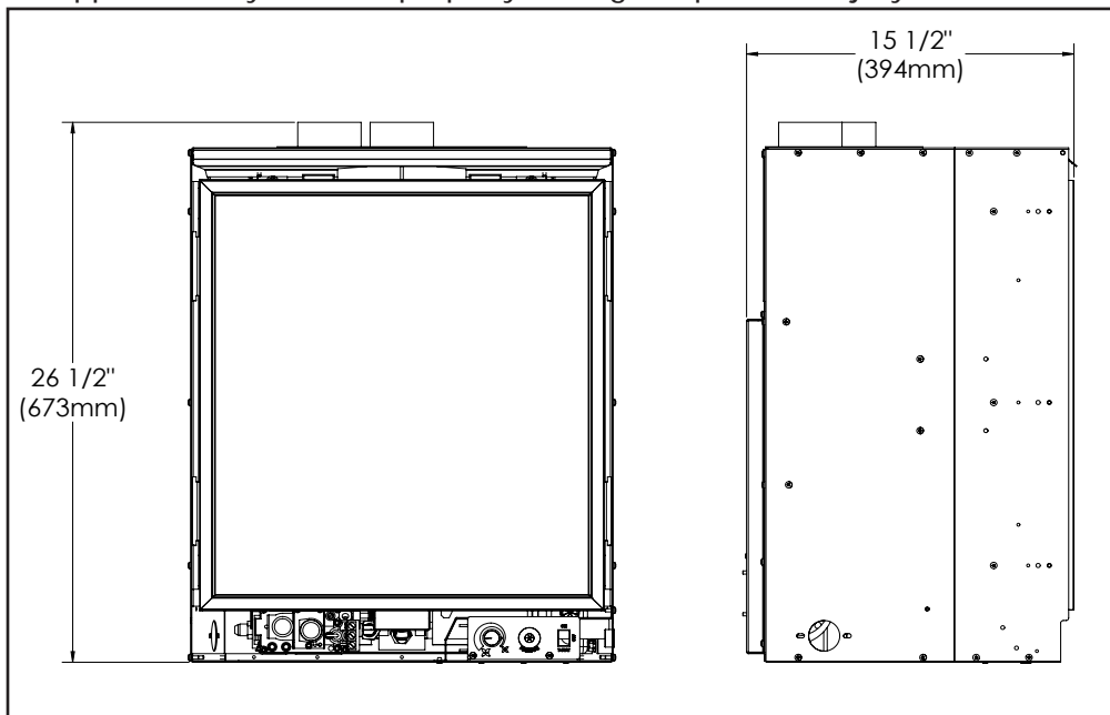
Figure 48: Q1 Insert Dimensions
