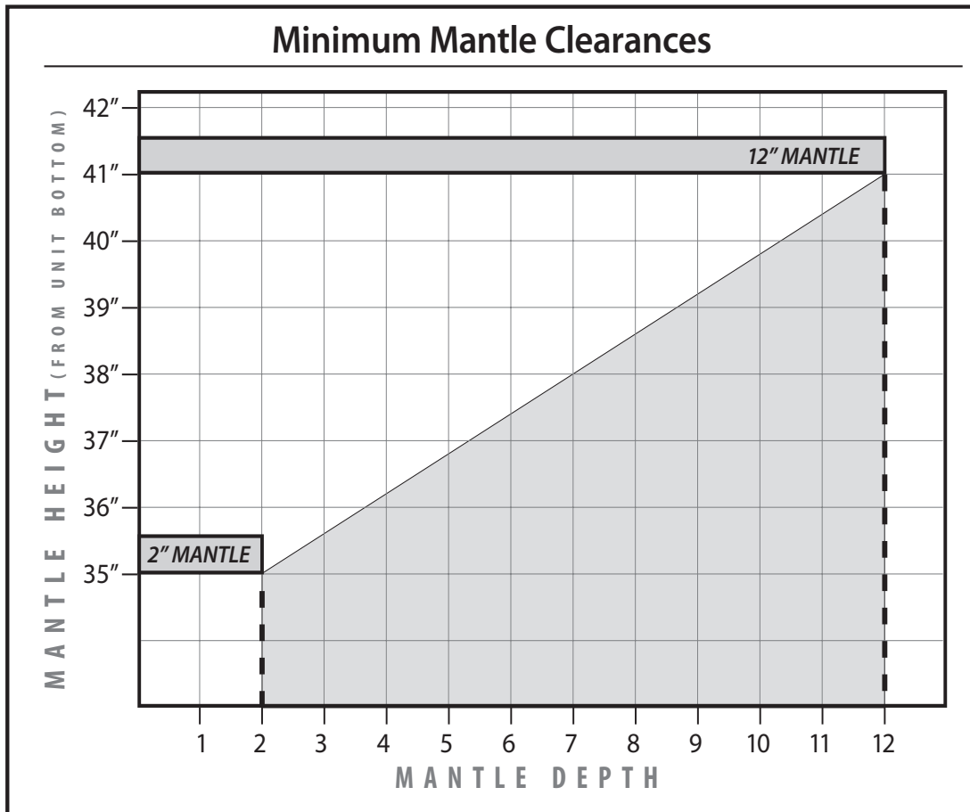
Figure 36: Mantle Clearances
