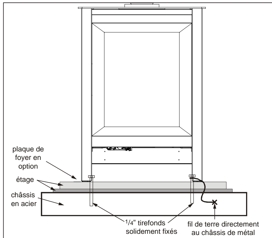
Figure 29: Installation de mobil-home
