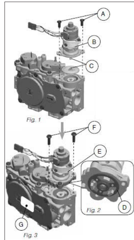
Figure 22: Conversion de la vanne SIT
