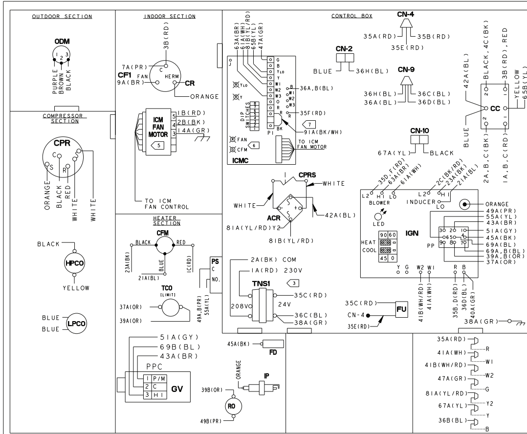
Figure 1. 4YCZ5024 and 4YCZ5048 Model Pg1
