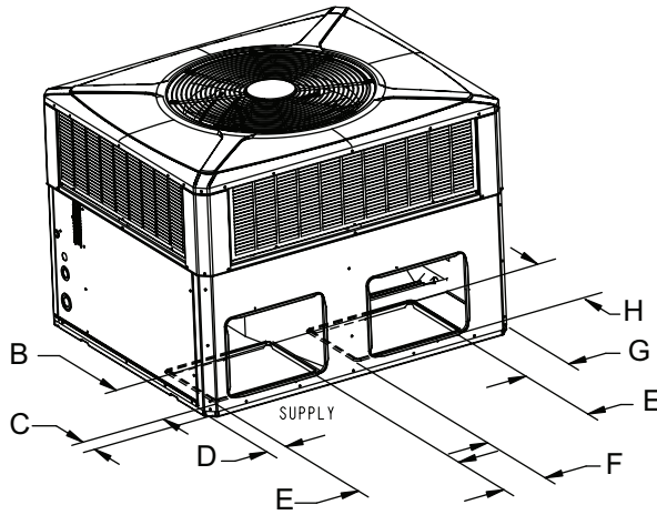
Figure 20. 2 - 5 Ton Models
