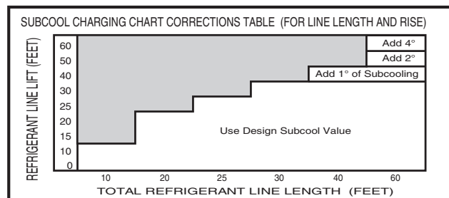
2 Ton Heat Pump
